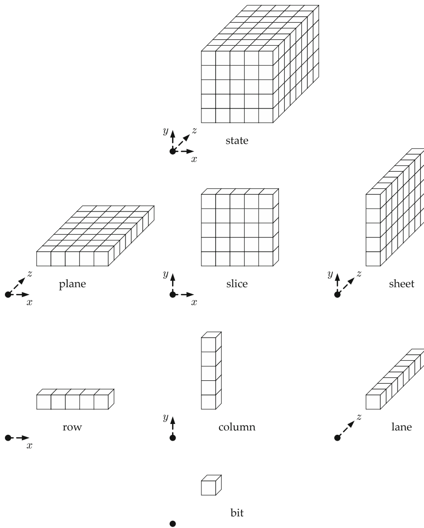
FIGURE 14.9. The SHA-3 state and its components
