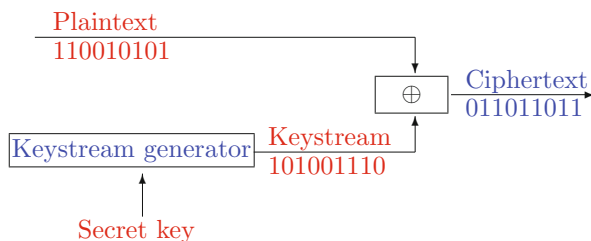
FIGURE 10.2. Stream ciphers
