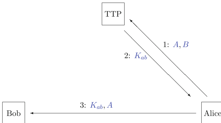
FIGURE 18.3. Protocol Version 1
