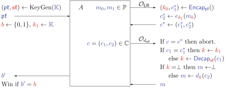
FIGURE 16.6. Game G_1
